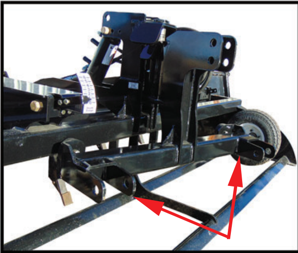
The Flex Hitch Swivels Left and Right making corners easy to negotiate.
