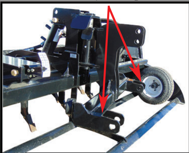
The Flex Hitch allows the Arena Quantum 2.5" of up and down movement, making the Quantum's travel independent of the tractor, eliminating bounce.
