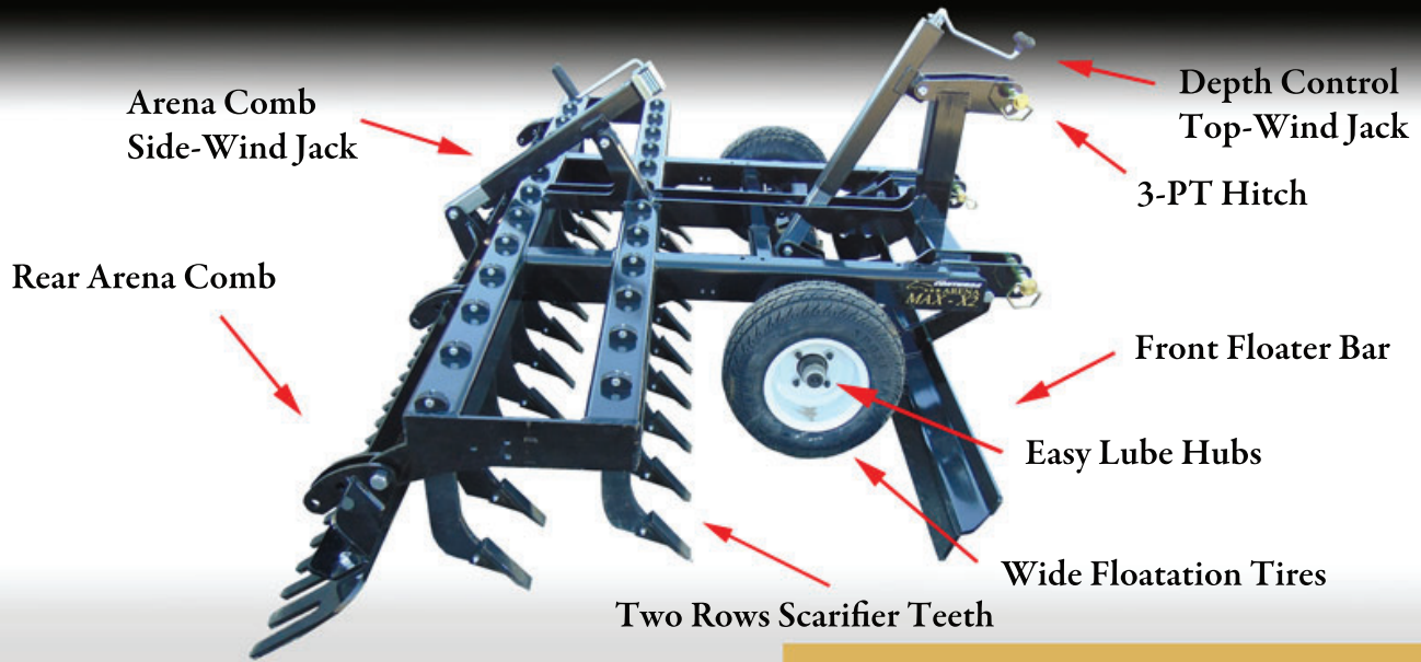
Two Rows of Easily Replaced Scarifier Teeth
