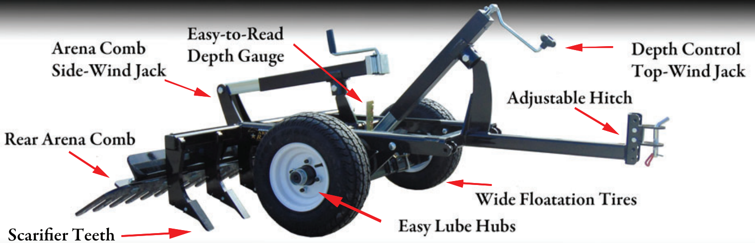
Scarifier Shank and durable, easily replaced Scarifier Teeth
