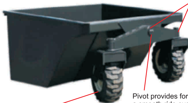
Large, heavy-duty pneumatic wheels allow for heavier loads
